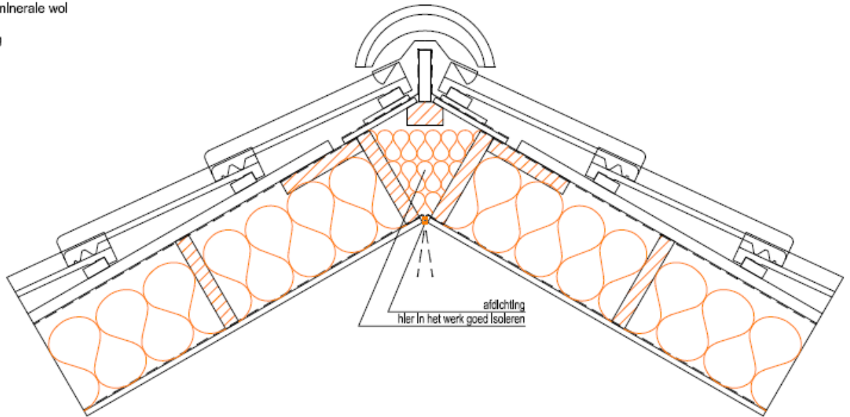
detail gordingen 4
